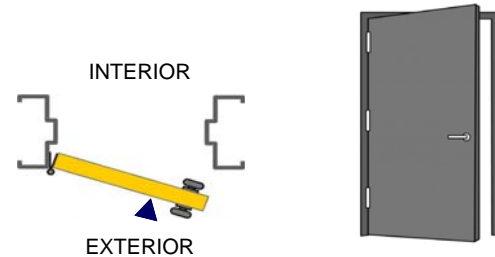
LEFT HAND REVERSE (Right Hand out-swing)
